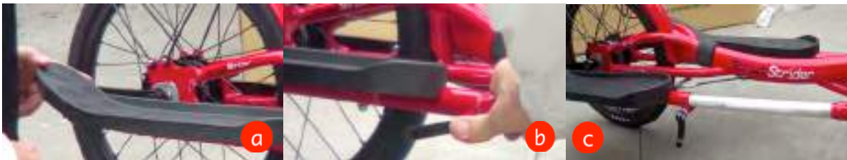
Figure 3B-6 a, b, c. Folding the JET for transport or storage
