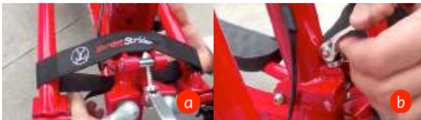
Figure 3B-2 a, b. Unfolding the JET
